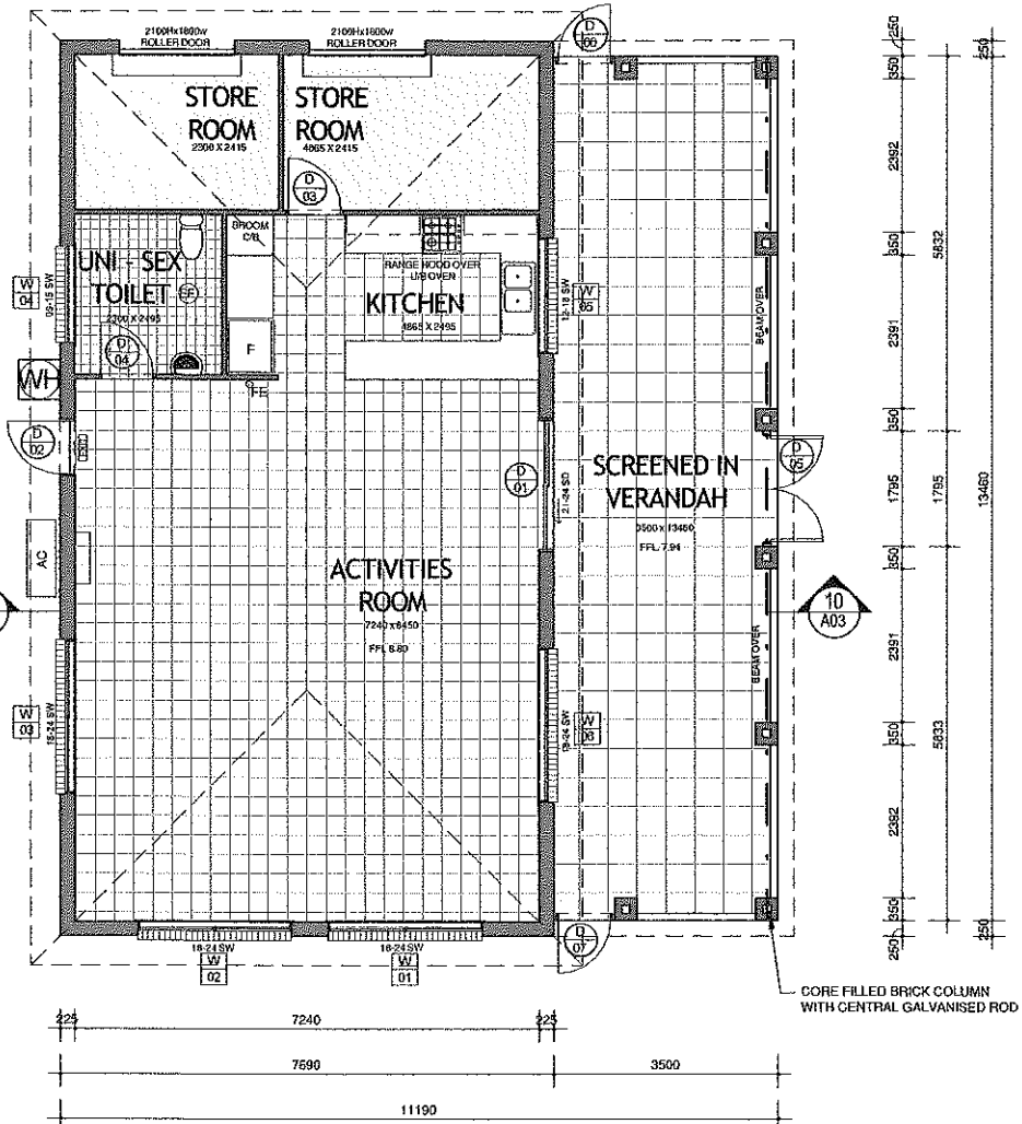
COMMUNITY HALL FLOOR - Plan
