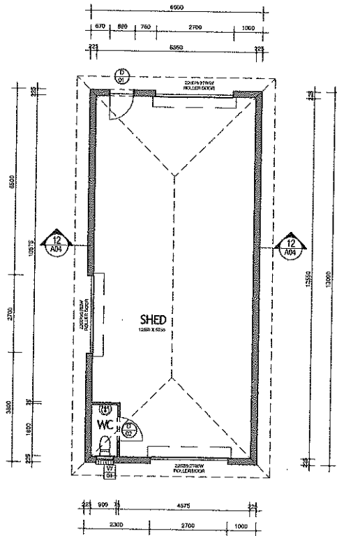
SHED FLOOR - Plan
